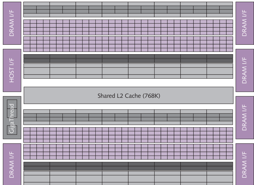
Figure 5. Fermi architecture block diagram. This top-level view of the architecture shows the 16 streaming multiprocessors, the six 64-bit DRAM interfaces, the host interface (PCI Express), and the GigaThread hardware thread scheduler.
