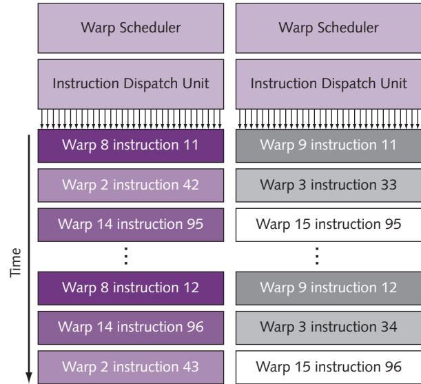
Figure 4. CUDA multithreading in the Fermi architecture. To achieve massively parallel multithreading, CUDA bundles 32 threads into a “warp” and executes one instruction from each thread per clock cycle. Each streaming multiprocessor can manage 48 warps. The warp schedulers and dispatch units interleave the threads and warps to keep the CUDA processor cores busy. The GPU can switch from one thread to another on each clock cycle.
