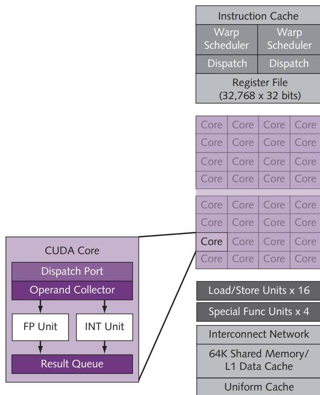
Figure 2. CUDA-core block diagram. CUDA cores evolved from pixel shaders, so they are very simple processor cores. The cores lack their own general-purpose register file, L1 caches, multiple function units for each data type, and load/store units for retrieving and saving data.
