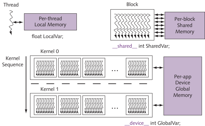
Figure 7. Memory allocation with CUDA. By using special CUDA keywords added to C, programmers can specify the memory regions in which variables store their data. This is important not only for scoping the variables, but also for keeping local data close to the CUDA processor cores. The wider the scope, the more distant the memory.
