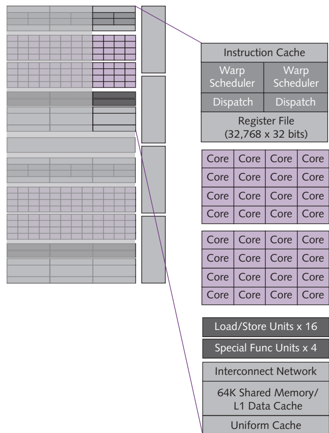
Figure 3. Streaming-multiprocessor block diagram. In the Fermi architecture, each streaming multiprocessor has 32 CUDA cores—four times as many as the previous GT200 and G80 architectures. All 32 cores share the resources of their streaming multiprocessor, such as registers, caches, local memory, and load/store units. The “special function units” (SFUs) handle complex math operations, such as square roots, reciprocals, sines, and cosines.
